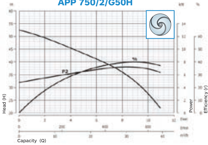
APP 750/2/G50H
