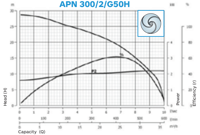
APN 300/2/G50H
